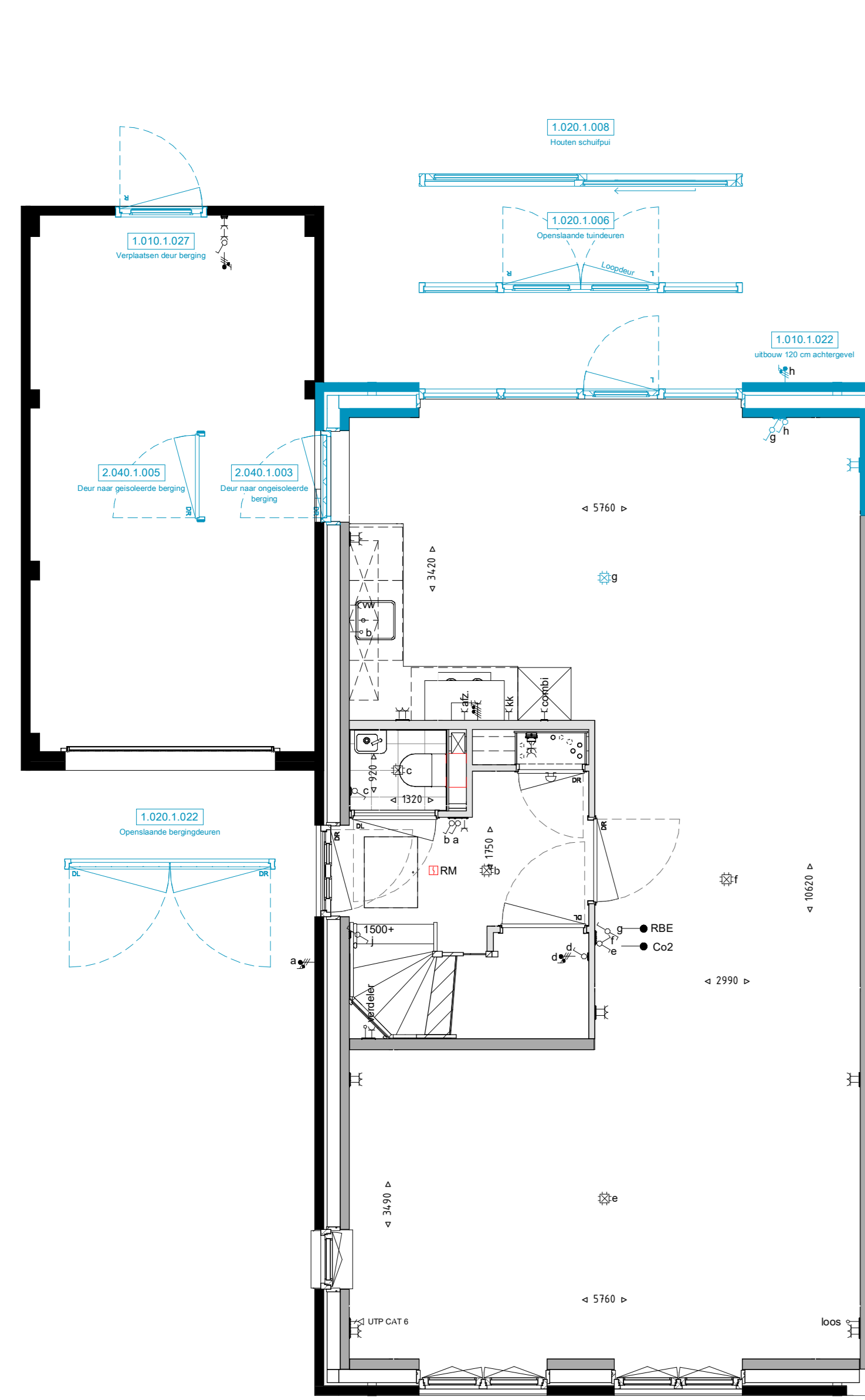
Begane grond 1: 50
