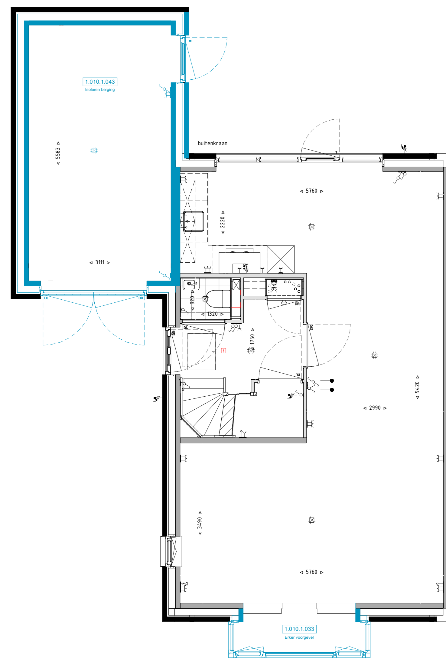
Begane grond 1: 50
